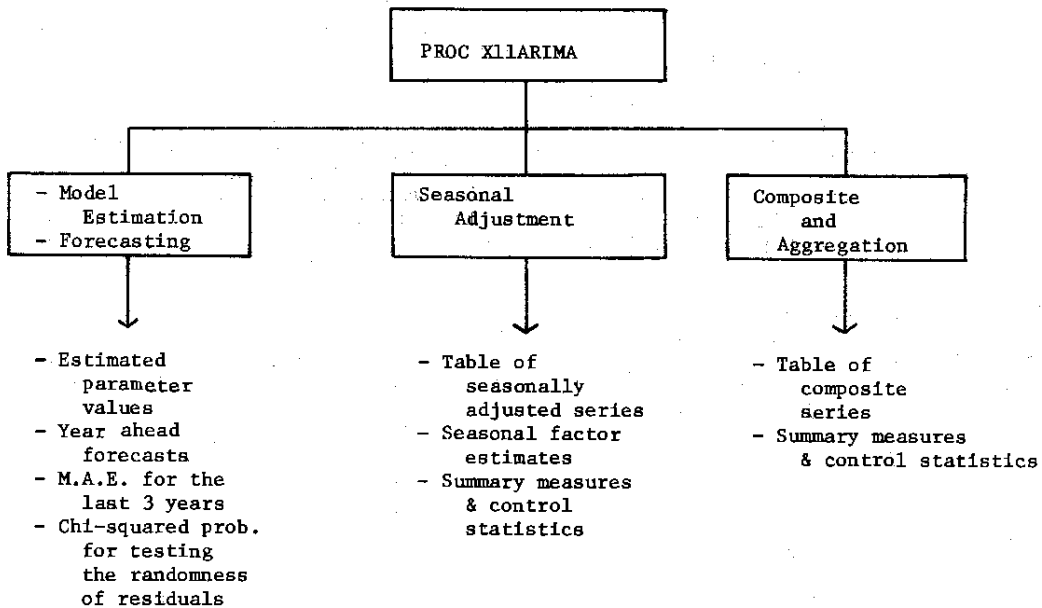
Figure 2. Basic Functions of PROC XLIARIMA
