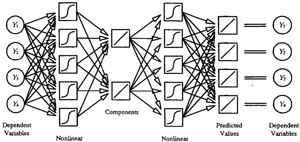
Figure 16: Nonlinear Analog of Principal Components
