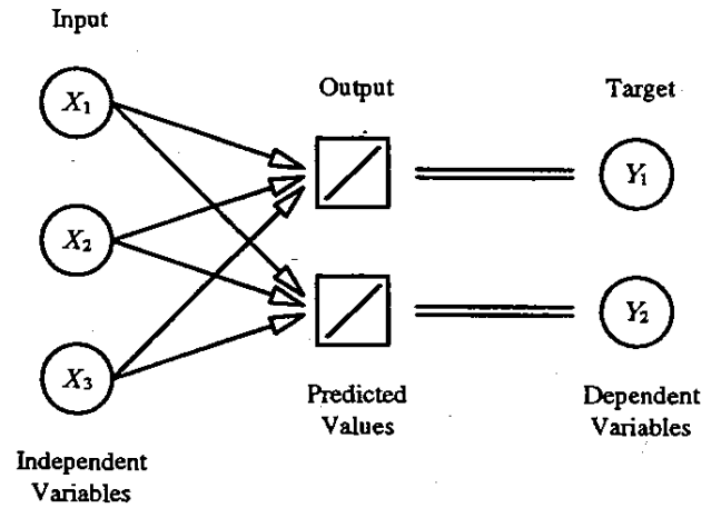
Figure 3: Simple Linear Perceptron = Multivariate Multiple Linear Regression
