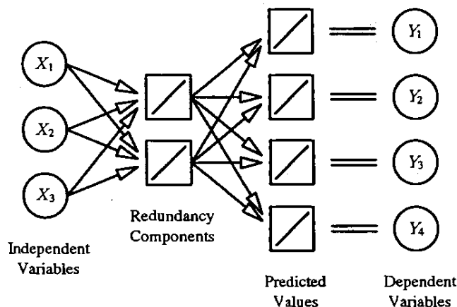
Figure 14: Linear Multilayer Perceptron = Maximum Redundancy Analysis
