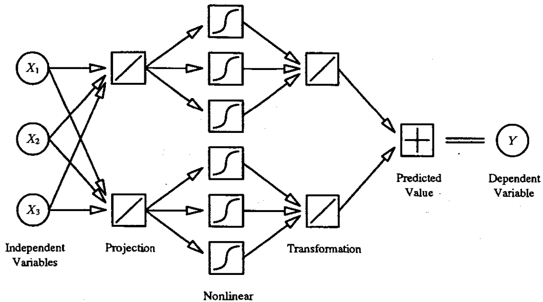
Figure 18: Projection Pursuit Network
