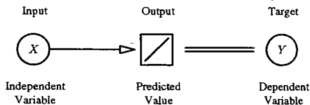
Figure 1: Simple Linear Regression
