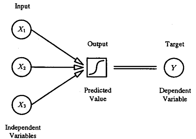
Figure 4: Simple Nonlinear Perceptron = Logistic Regression
