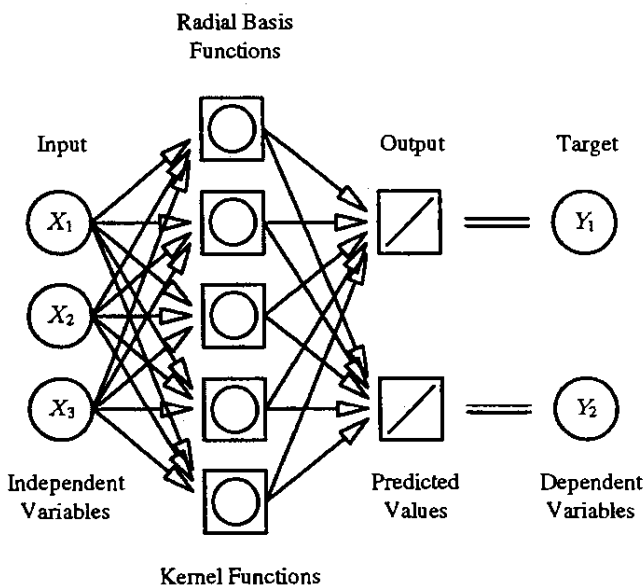
Figure 13: Radial Basis Function Network
