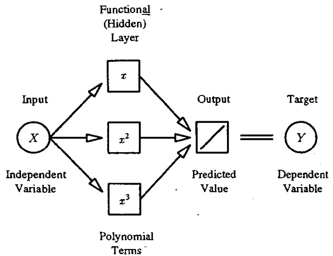
Figure 6: Functional Link Network = Polynomial Regression
