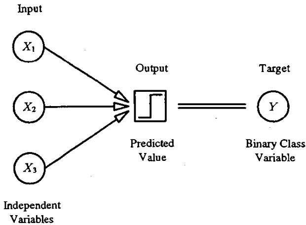
Figure 5: Adaline = Linear Discriminant Function
