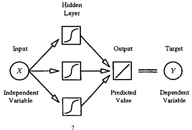
Figure 7: Multilayer Perceptron = Simple Nonlinear Regression
